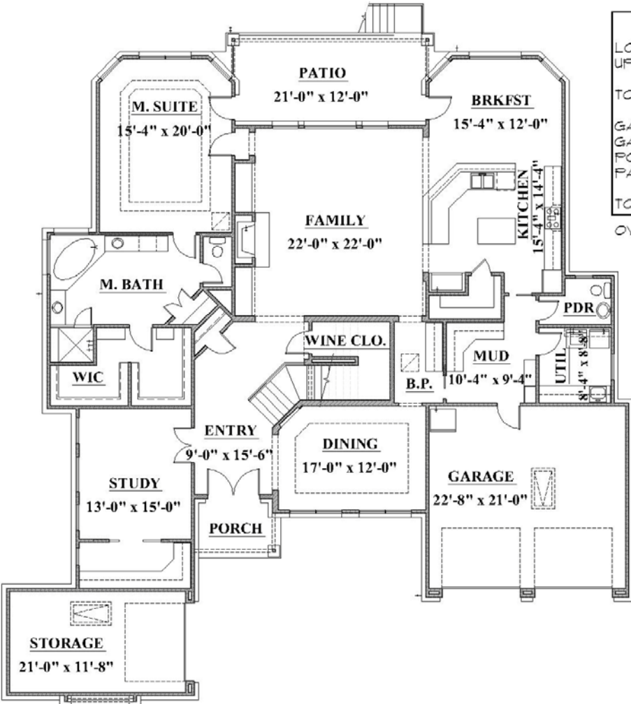
LOWER FLOOR PLAN 00043-P
