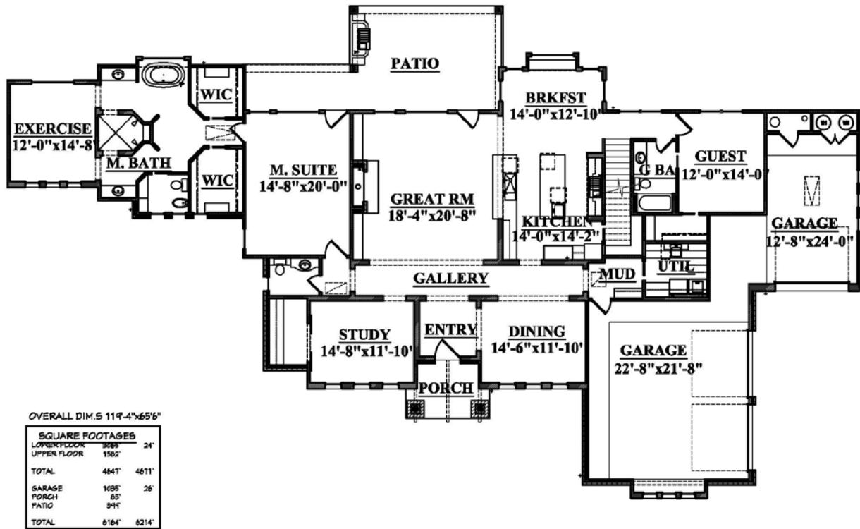
LOWER FLOOR PLAN 12221 MUSKET RIM
